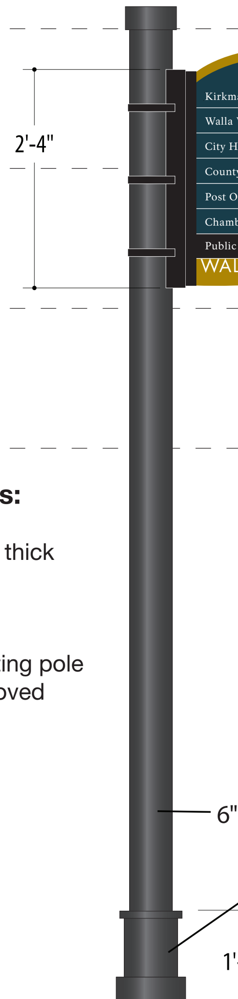
PDIR.2 Pedestrian Directional (New Pole)
