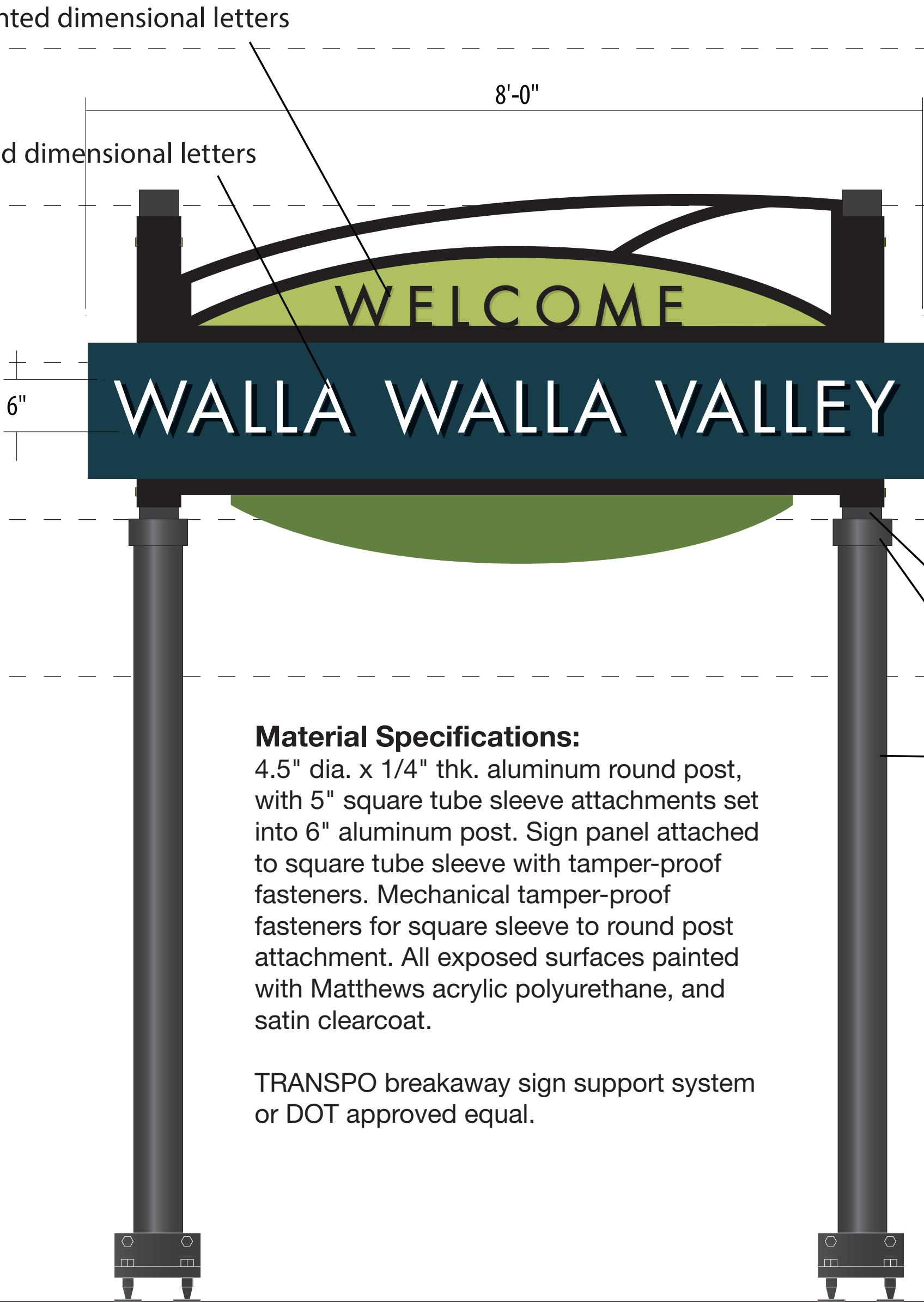
GATE.2 Secondary Valley Gateway
